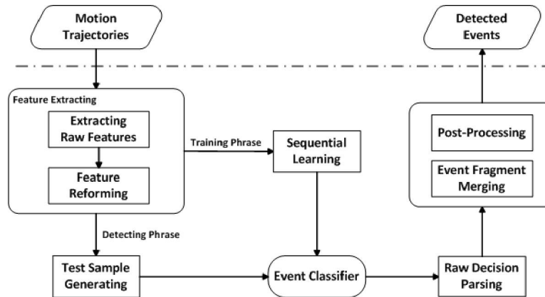
Fig.4. Flowchart of sequential learning based event detection
