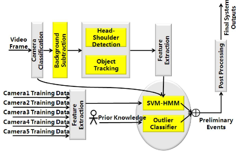
Fig.1. Diagram of our system, eSur
