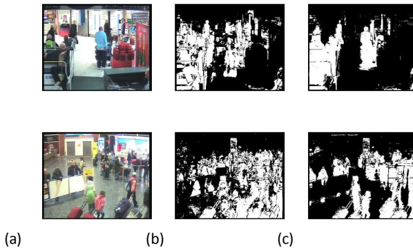
Fig.5 Background subtraction results. (a) video frame (b) result with classic eigenbackground (c) result with proposed method
